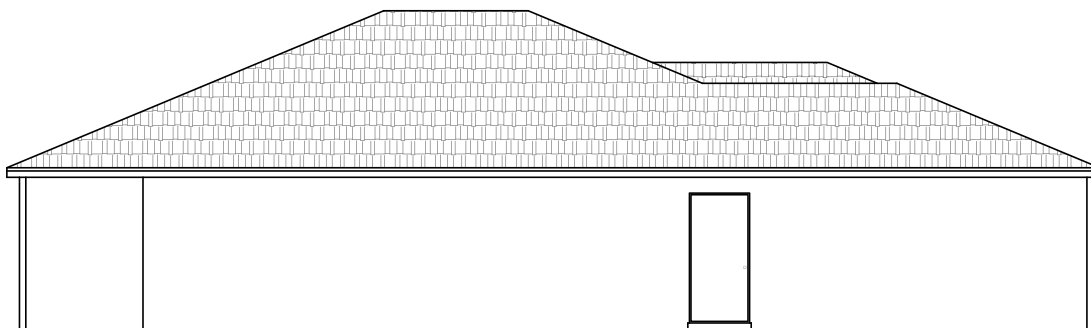
Left Elevation
