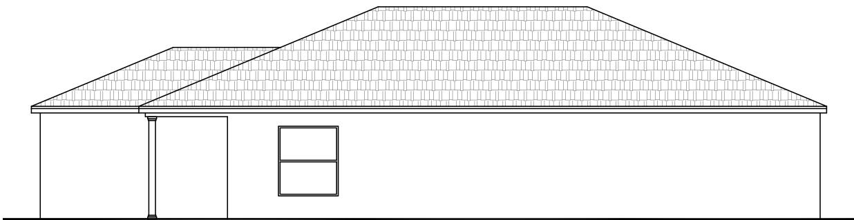
Right Elevation 58'8"
