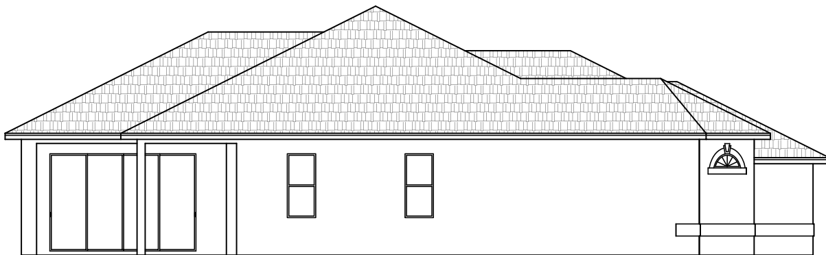
Left Elevation
